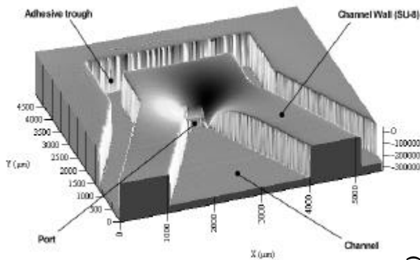
Figure 5. Profile of one end of μ-TFFF. The power is more than 1000 times lower than that reported for a typical macro-scale TFFF channel. Plate height was determined as a function of average carrier velocity and compared with results from the μ-EFFF system [33] and
