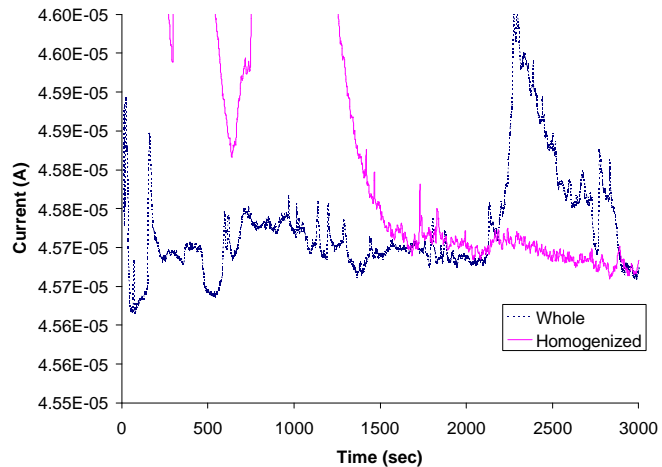
Figure 13. Comparison of whole blood and homogenized blood retained in the \mu -EFFF system focusing on the whole blood fractogram. Notice there is continual elution of particles during most of the run, but a strong peak appears near the end of the run in a range where no elution in the homogenized sample occurred.
