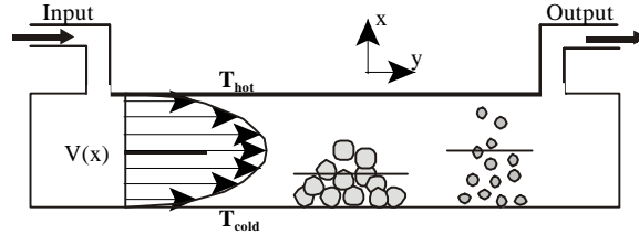
Figure 4. Schematic of a thermal field-flow fractionation (TFFF) channel.
